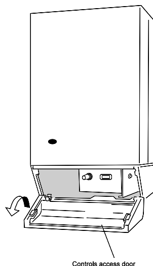
Standard Model
